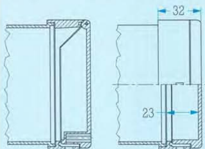
Door and frame for plastic cases
